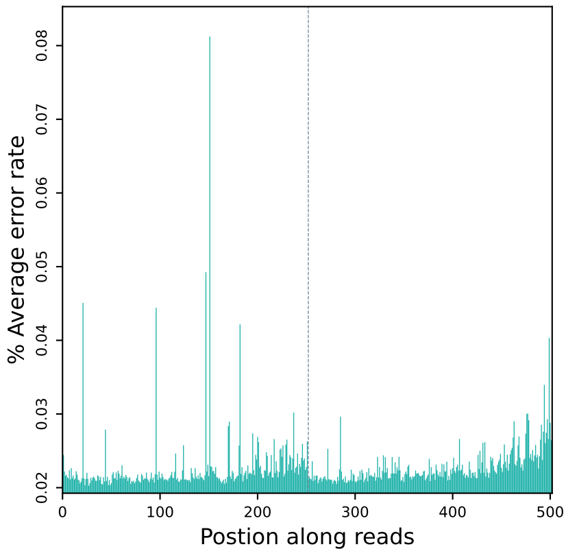
Error rate distribution along reads (R10502)
